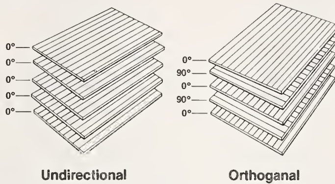
Examples of laminate ply construction when using SMC-C
